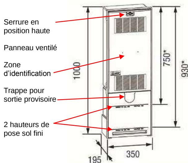
Borne
